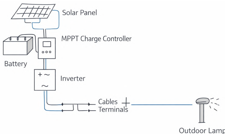
Figure 3. Block Diagram of a Centralized Solar-Powered Outdoor Lighting System
